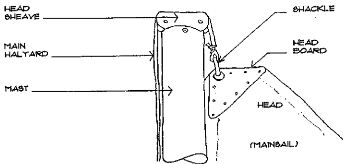
JY-15 (A) Top Mast Detail (PORT SIDE)
